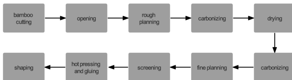
Figure1 Holse & Wibroe semi-finished bamboo manufacturing process
