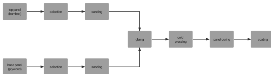
Figure 1 Holse & Wibroe bamboo wood composite manufacturing process
